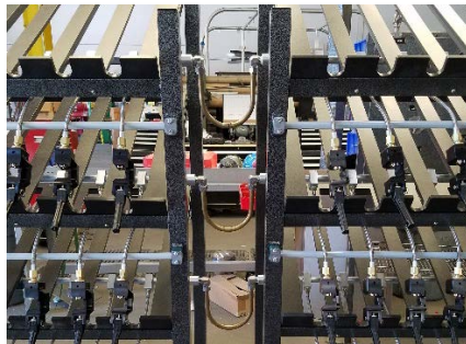
Rack Modular Connectivity between R30 Racks No Isolation valves
