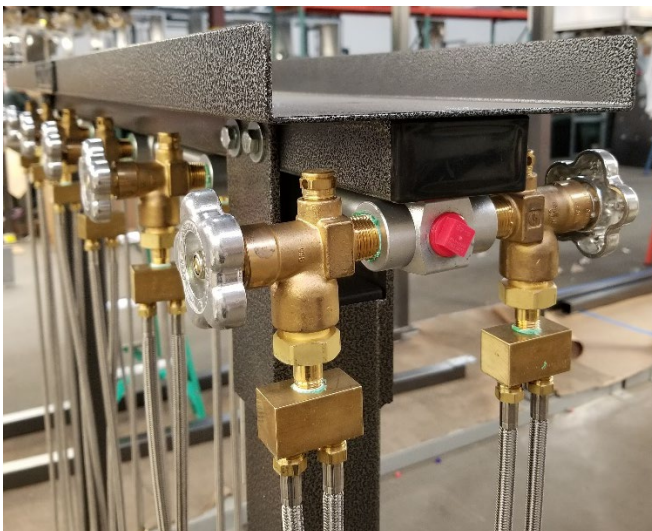
Left: Shows the modular connection with dual pigtail station valves with tee and CGA fittings
